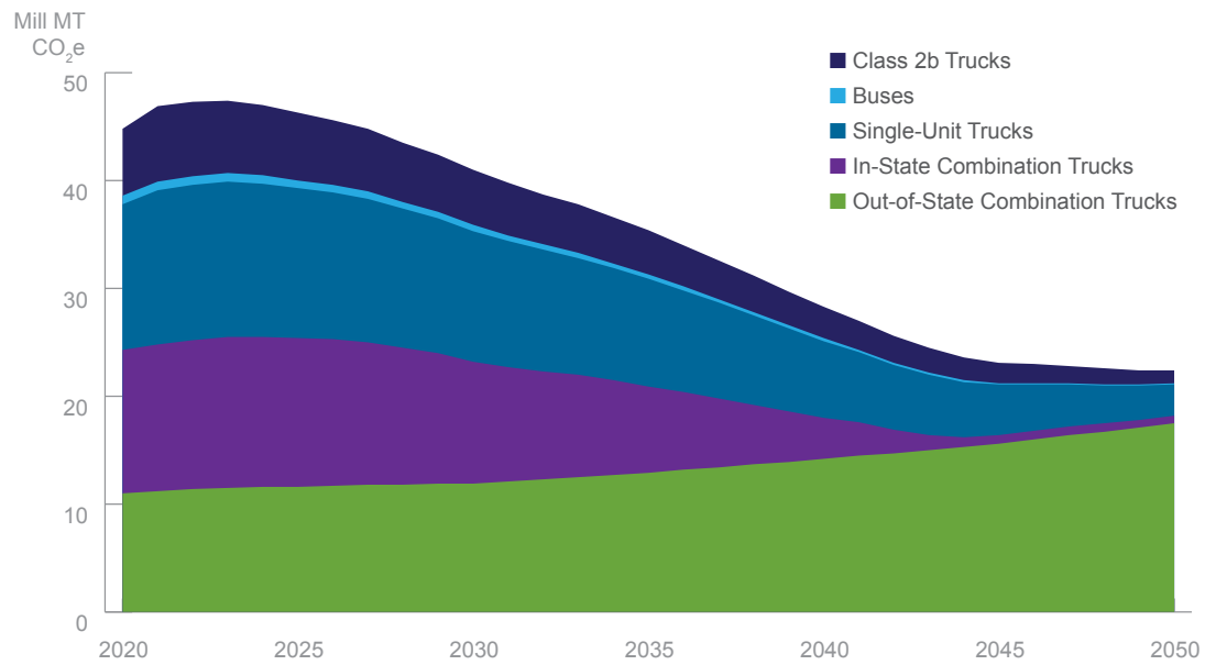
Figure A6 GHG Emissions Under “100% Sales by 2036” Scenario by Vehicle Category
